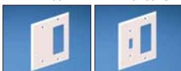
MP2GRB
